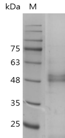
SDS-PAGE analysis of recombinant human HMGB1 C23AC45AC106A
